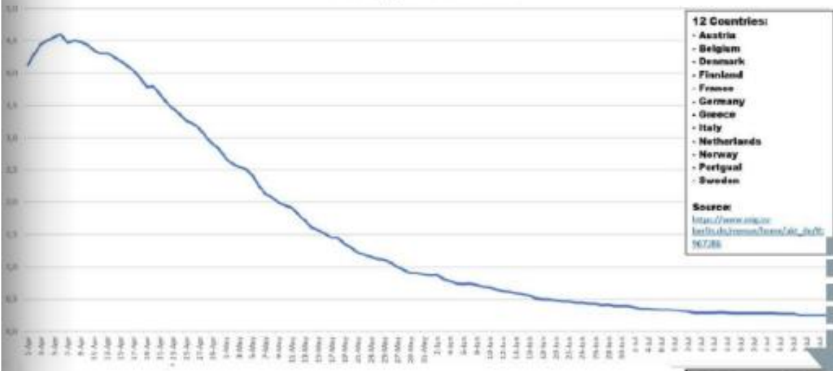
Covid-19 current ICU / 100.000 population 12 european countries
